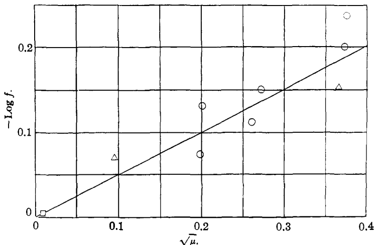
Fig. 3.—Activity coefficients of 5-phenyl-10-methylacridinium hydroxide: ○, added salt—KCl; △, added salt—BaCl 2 ; □, no added salt.
