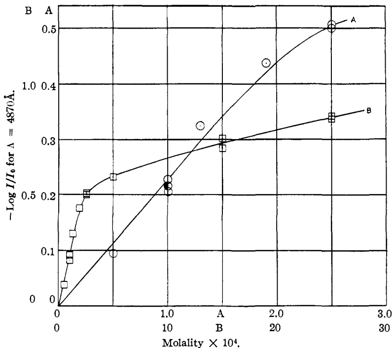
Fig. 2.—Curves used in the analysis of 5-phenyl-10-methylacridinium chloride solutions: points on Curve A, \odot (no added salt); \bullet ( 0.26 M in KCl); points on Curve B, \square (no added salt).
